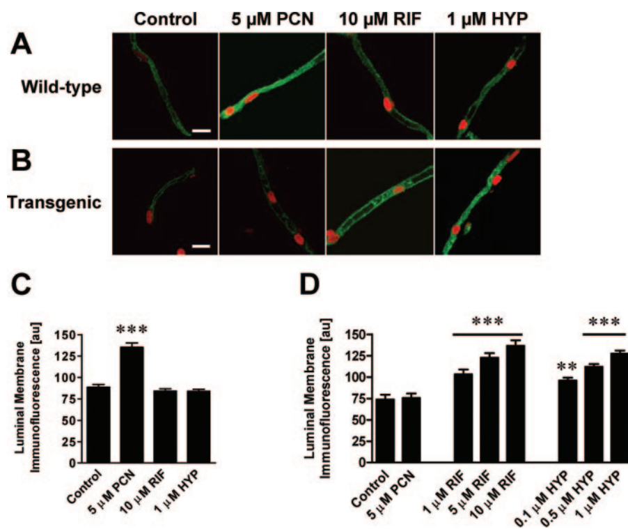
Fig. 2. P-glycoprotein expression in brain capillaries after exposure to PXR ligands. A, representative images showing immunostaining of P-glycoprotein in isolated brain capillaries from wild-type mice. Exposing brain capillaries for 6 h to PCN increased P-glycoprotein expression; rifampin (RIF) and hyperforin (HYP) had no effect (scale bar: 10 \mu m). B, representative images showing immunostaining of P-glycoprotein in isolated brain capillaries from hPXR transgenic mice. Six-hour exposure of rifampin and hyperforin, but not PCN, increased P-glycoprotein expression in capillaries of hPXR transgenic mice (scale bar: 10 \mu m). C, quantitation of luminal membrane P-glycoprotein immunofluorescence from capillaries of wild-type mice exposed to PCN, rifampin, or hyperforin. D, concentration-dependent increase of luminal membrane P-glycoprotein immunofluorescence from isolated capillaries of hPXR transgenic mice exposed to rifampin or hyperforin; PCN had no effect. Each bar represents the mean value (arbitrary fluorescence units, scale 0–255) of 15 to 20 capillaries from a single preparation (pooled tissue from five wild-type mice or three hPXR transgenic mice); variability is given by S.E. bars. Statistical comparison: **, significantly greater than control, P < 0.01; ***, significantly greater than control, P < 0.001.
